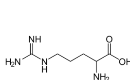
Arginine
